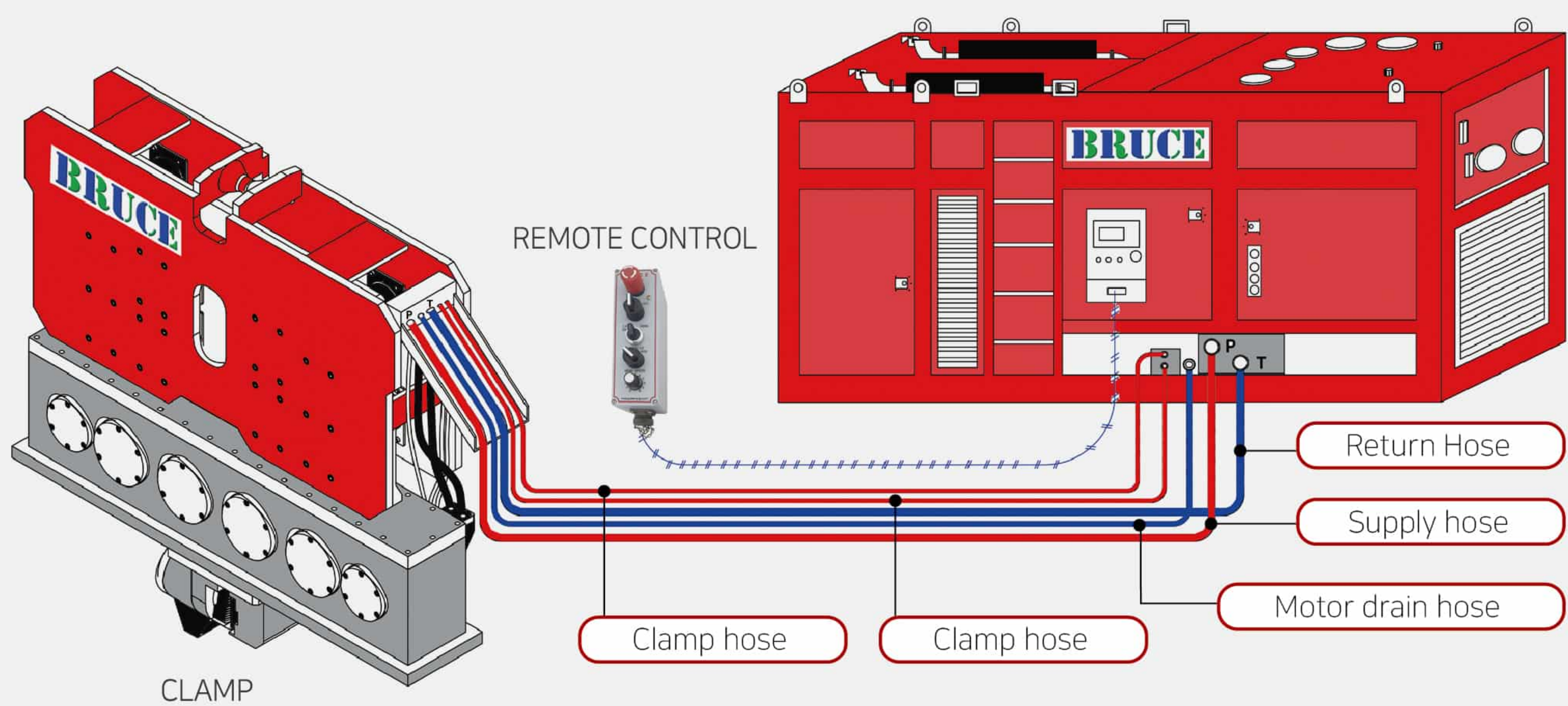
HYDRAULIC VIBRO HAMMER
