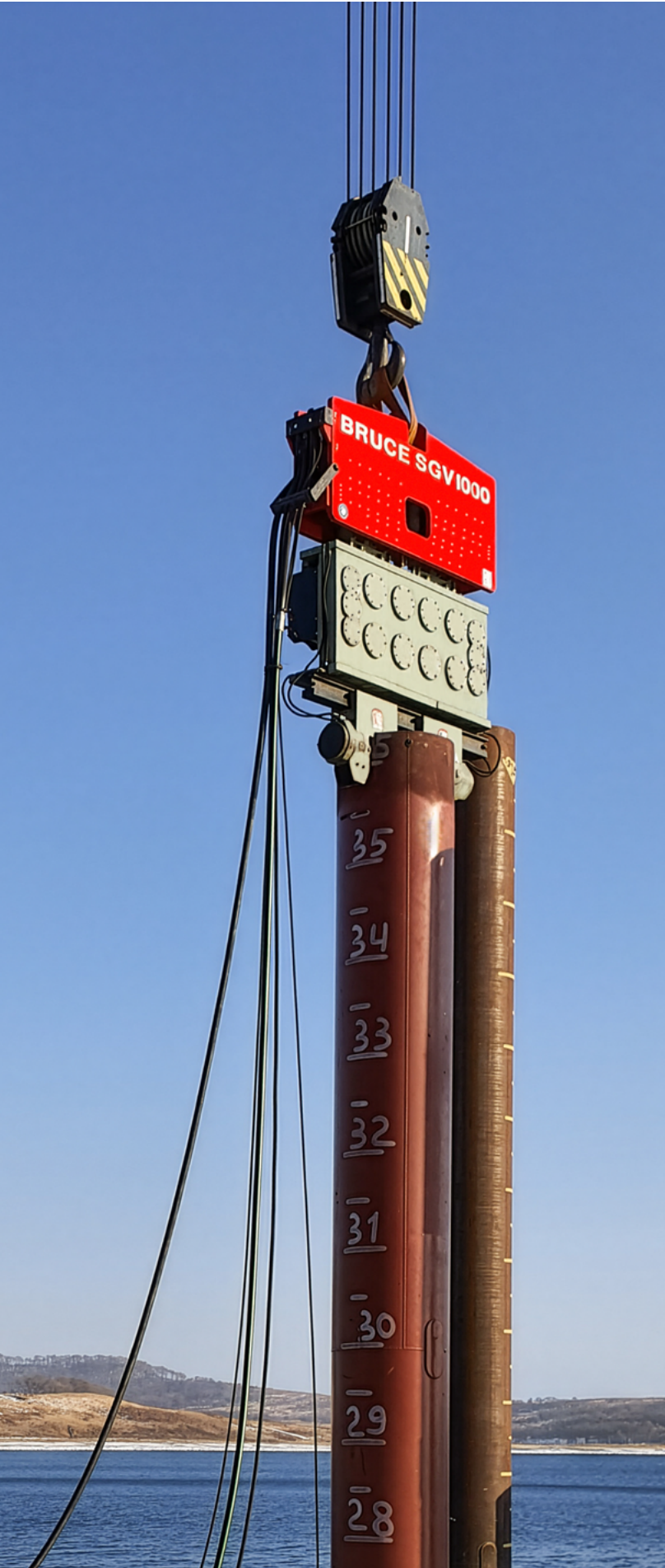
BRUCE Vibratory Hammer SGV 1000
