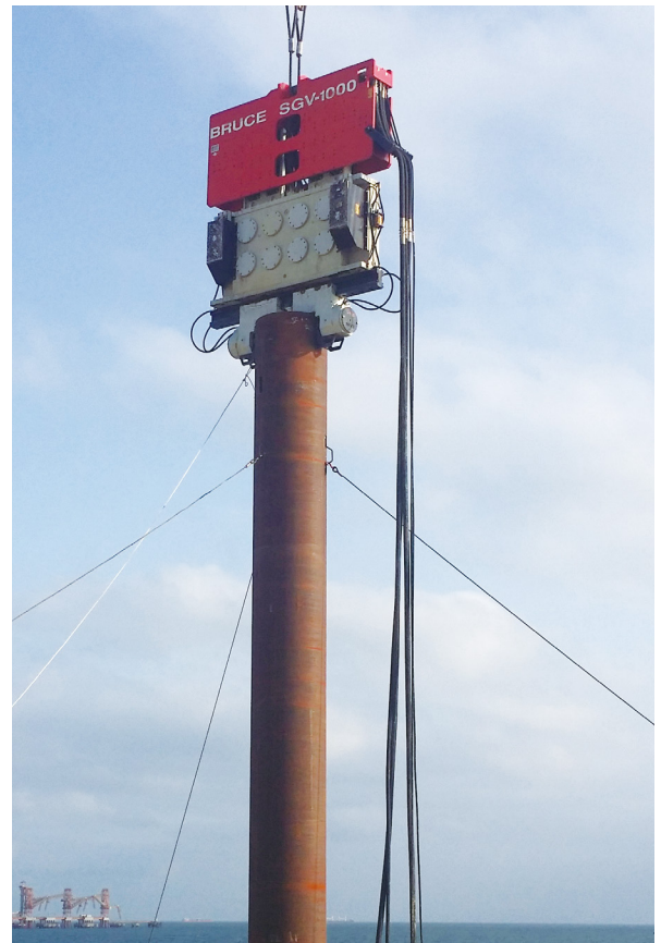
BRUCE Vibratory Hammer SGV 1000
